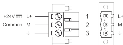
Fig. 13: Power connector TX7...
