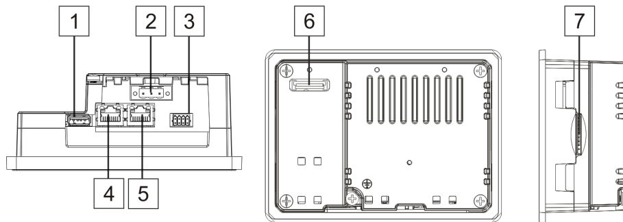
Fig. 11: TX705 – connectors
