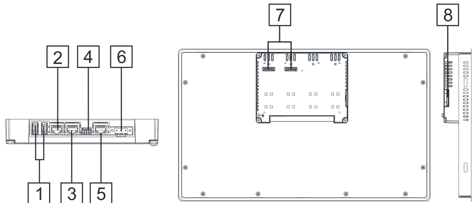
Fig. 12: TX707... TX721 – connectors
