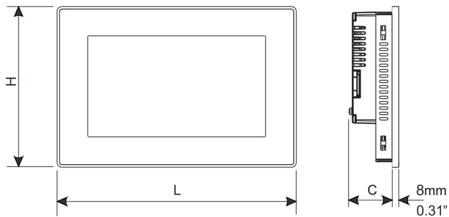
Fig. 5: Dimensions – TX710(HB), TX715, TX721
