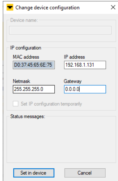
Fig. 20: Turck Service Tool – changing the IP configuration
