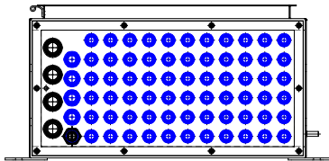
FLANGE VIEW
