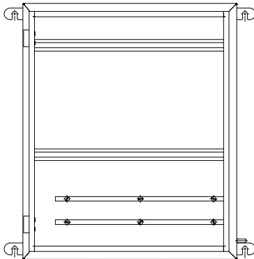
MOUTING VIEW
