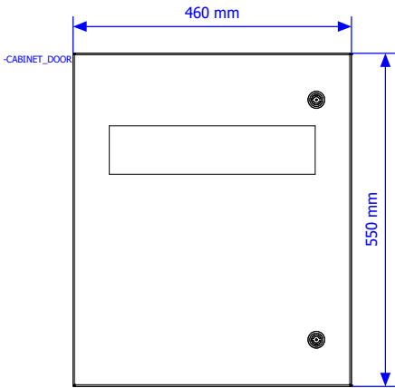
DOOR VIEW
