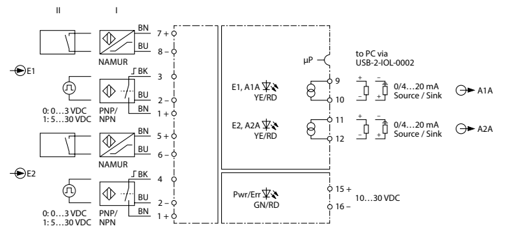
IM12-FI01-2SF-2I-C0/24VDC/K71
