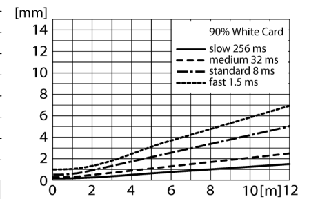
Caracteristica "Excess gain"
